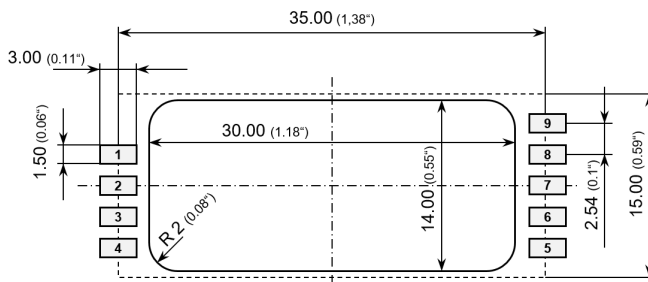
Recommended PCB footprint
